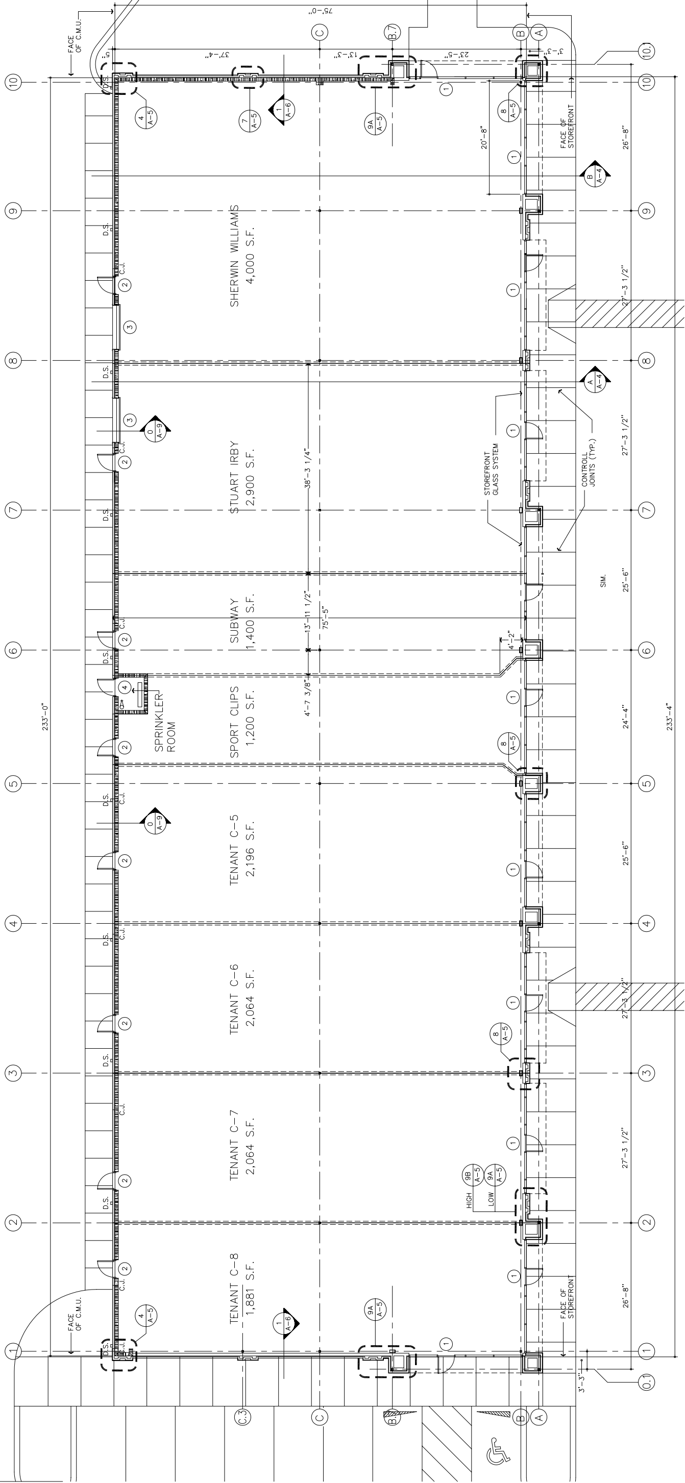
FLOOR PLAN
